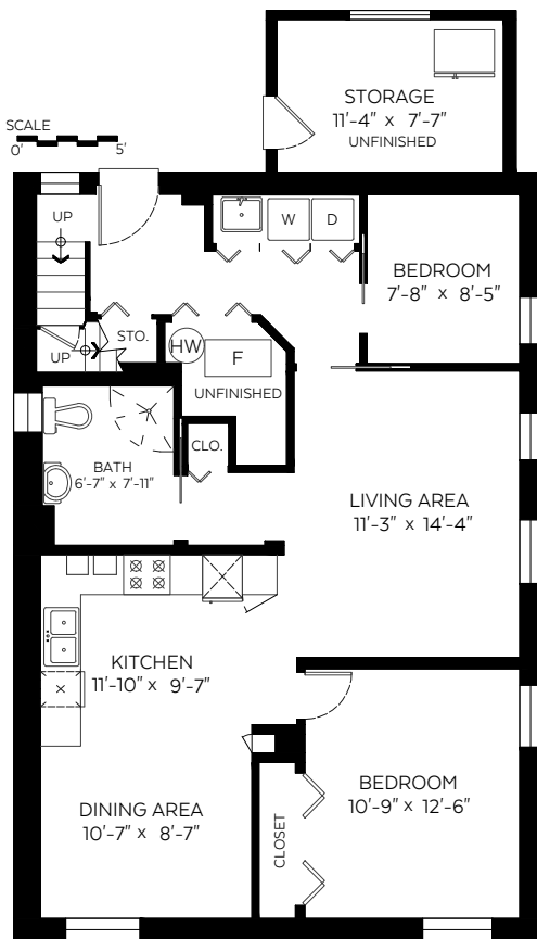
Lower Floor Plan Floor Area: 1,012.ft
